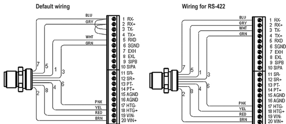
Figure 2 Internal Wiring
